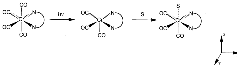
Fig. 2. Dissociative photochemical substitution of \text{Cr}(\text{CO})_4(\text{bpy}) . The coordination of the solvent molecule S probably starts at later stages of the CO dissociation. In the presence of a Lewis base L, the \text{Cr}(\text{S})(\text{CO})_3(\text{bpy}) photoproduct undergoes another, thermal, substitution to form \text{Cr}(\text{L})(\text{CO})_3(\text{bpy}) as a stable product. Typically, L = phosphine or phosphite. The axes orientation shown is used throughout this paper.
